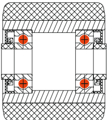
Labyrinth sealing
