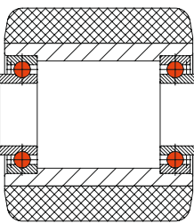
ZZV-ball bearing
