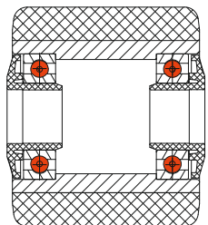
KS-sealing
