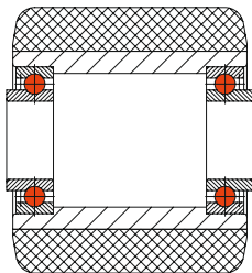
ZZV-ball bearing
