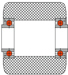
ZZV-ball bearing
